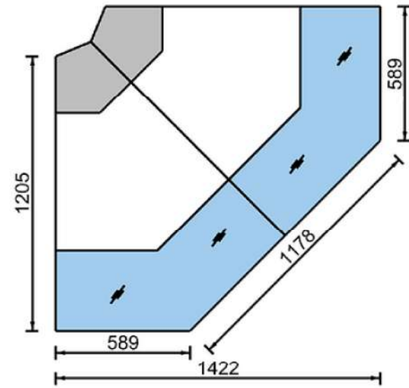
Mires 2 92S - External Corner (90°)
