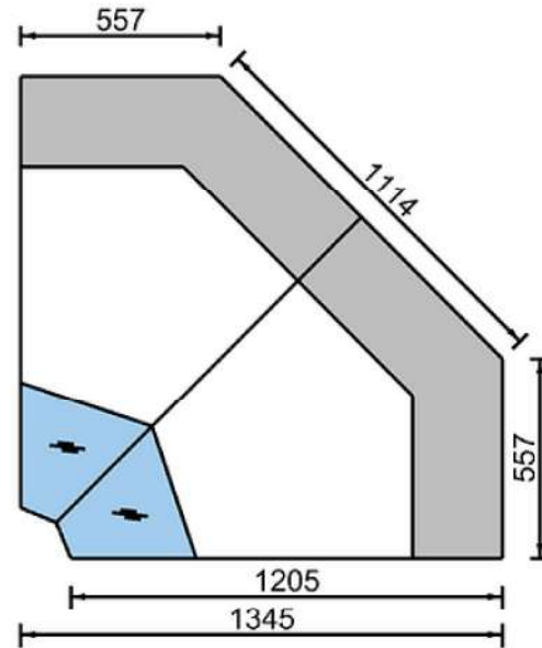
Mires 2 92S - Internal Corner (90°)
