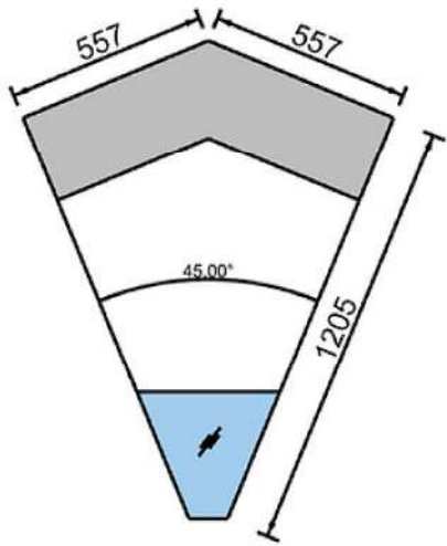
Mires 2 92S - Internal Corner (45°)
